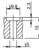
ASSEMBLY SCREWS SEAT ] x2
