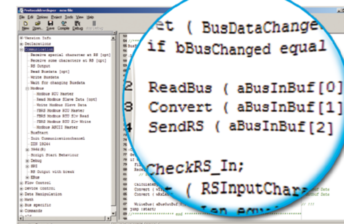
Script example in the Protocol Developer
